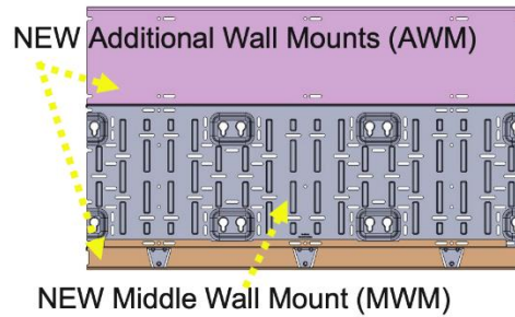
New 3-Piece Assembly (UL9540A Compliant)
