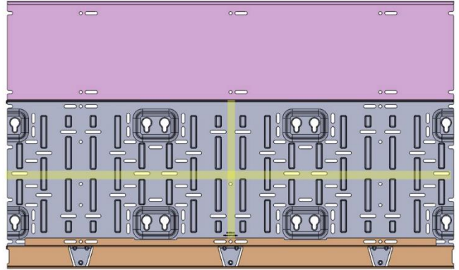
UL9540A Design (3-piece Bracket; New Wall Mount Assembly)
