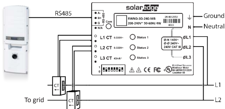
Connecting the Electricity Meter
