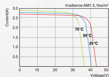
SLP085-24U I-V Curves
