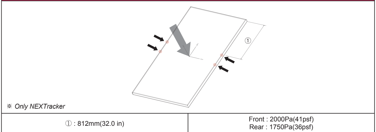
Fig7. Bolting Type
