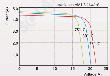
SLP080-12U I-V Curves
