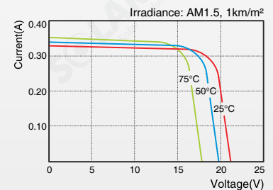
SLP005-12R I-V Curves
