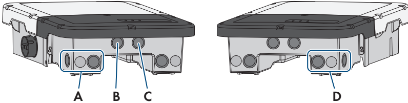
Figure 7 : Enclosure openings at the bottom of the inverter
