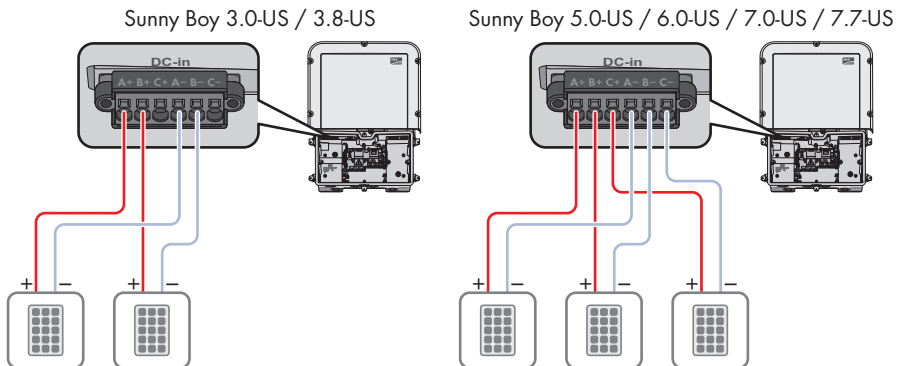
Figure 12 : Connection overview for normal operation
