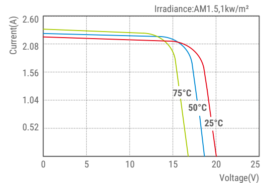
SLP030S-12U I-V Curves
