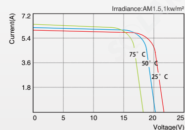
SLP100-12M I-V Curves
