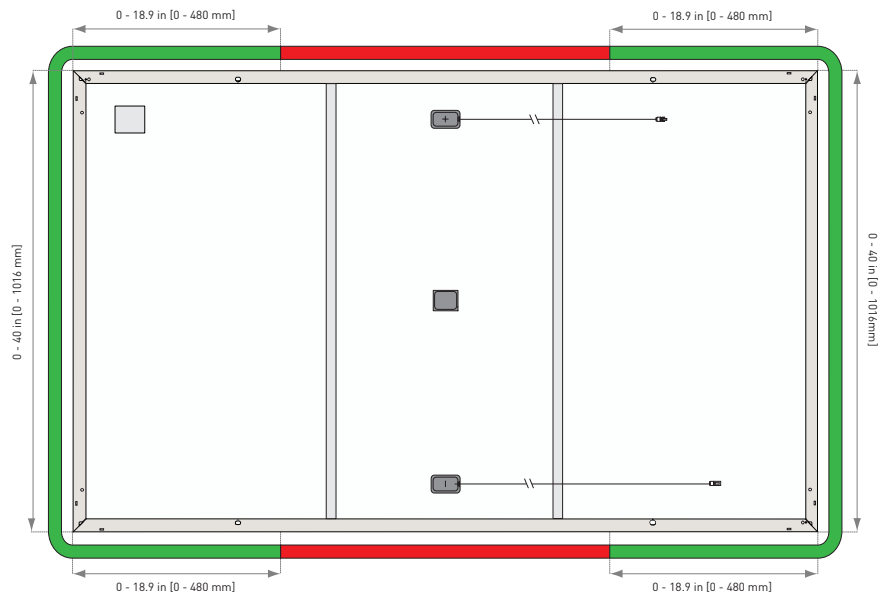
Figure 24. MLPE device installation zones
