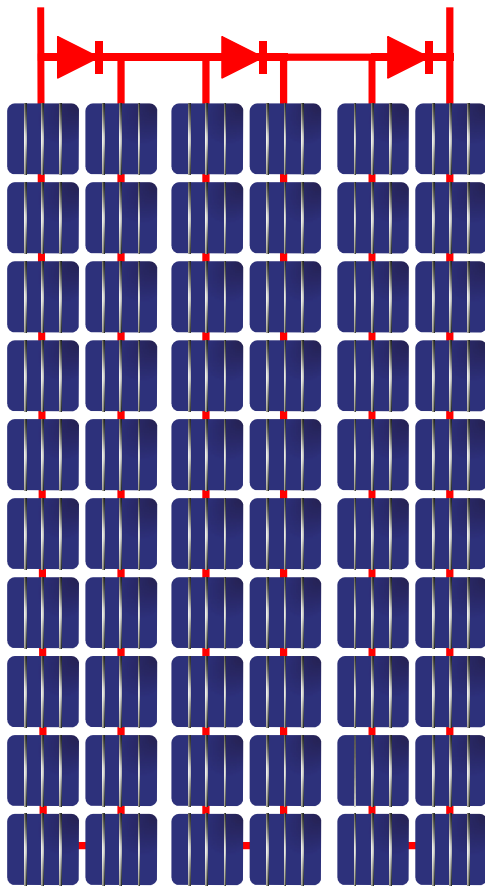
Figure 3: Cell inter-connection in a conventional series-connected panel.
