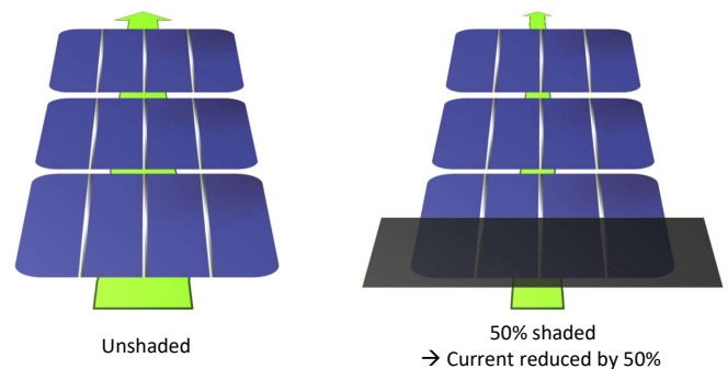
Figure 2: Shading a single cell reduces the current for the entire string.
