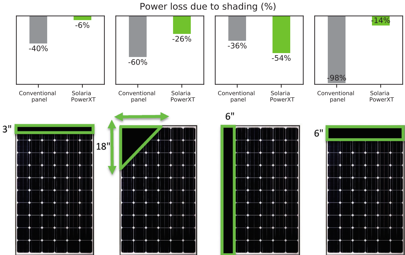
Figure 5: Measured power loss in four shading scenarios.
